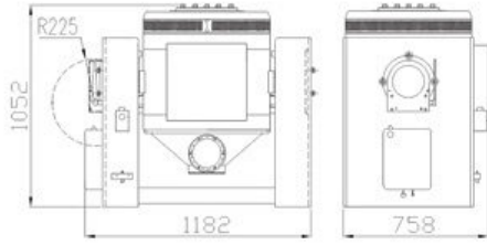
Shaker ET-20-320
